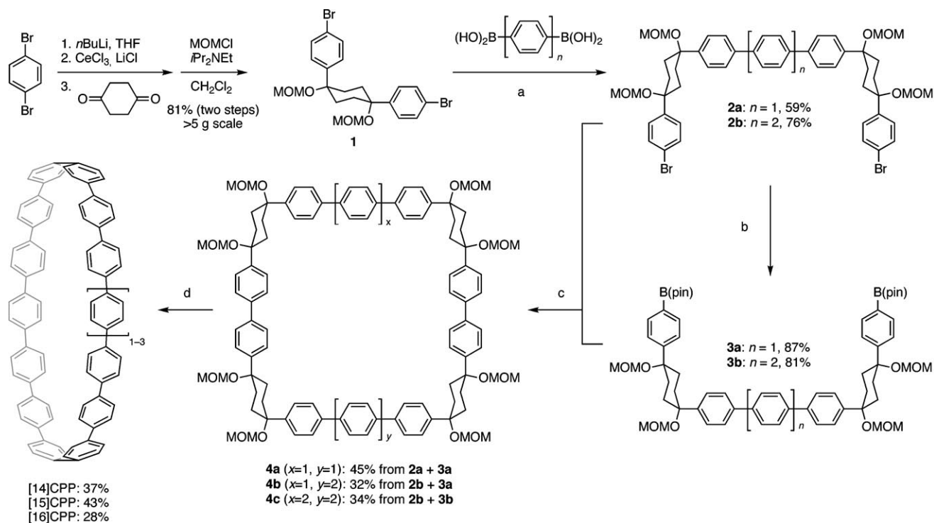
Scheme 3. Synthesis of [14] -, [15] -, and [16] CPP. Conditions and reagents: a) [\text{Pd}(\text{PPh}_3)_4] , \text{Na}_2\text{CO}_3 , n\text{Bu}_4\text{NBr} , \text{H}_2\text{O} , THF, 60^\circ\text{C} ; b) (pin)BB(pin), [\text{Pd}_2(\text{dba})_3] , X-Phos, KOAc, 1,4-dioxane, 90^\circ\text{C} ; c) \text{Pd}(\text{OAc})_2 , X-Phos, NaOH, \text{H}_2\text{O} , 1,4-dioxane, 80^\circ\text{C} ; d) \text{NaHSO}_4 \cdot \text{H}_2\text{O} , m -xylene, DMSO, reflux, under air.
